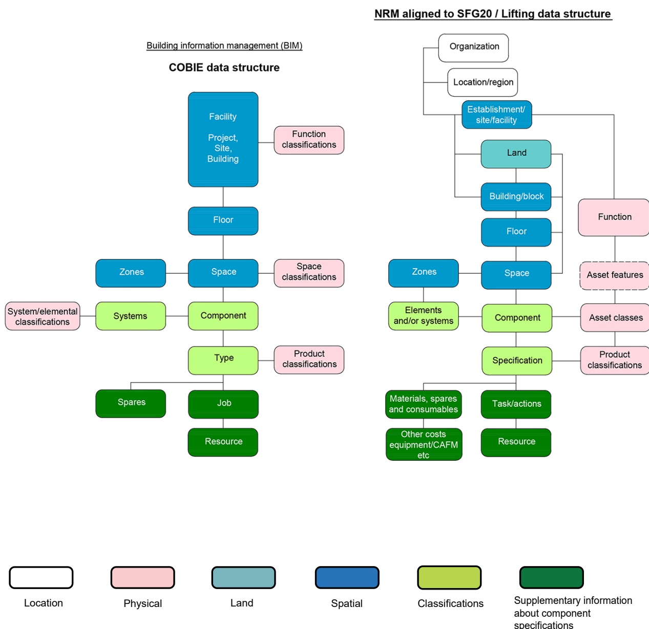
Figure 5: Alignment of NRM costs data structure [1] with COBIE data structure (BIM)
