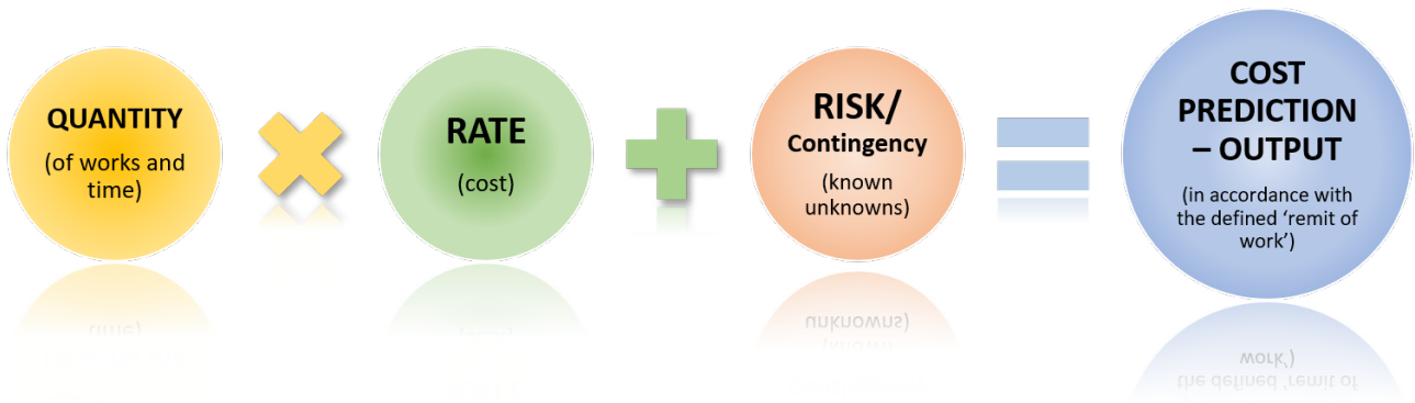
Figure 6: Transformational process
