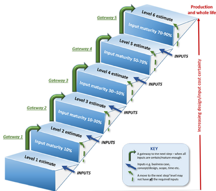
Figure 3: Information stages
